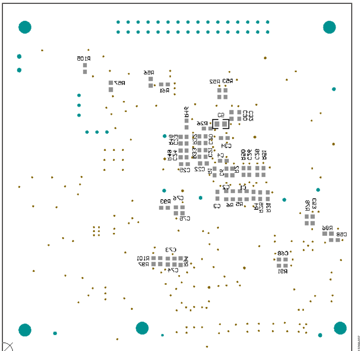
Figure 37. Analog Control Board Bottom Silkscreen
