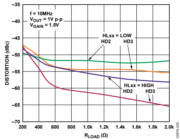
Figure 25. Harmonic Distortion vs. R_{LOAD} (See Figure 53)
