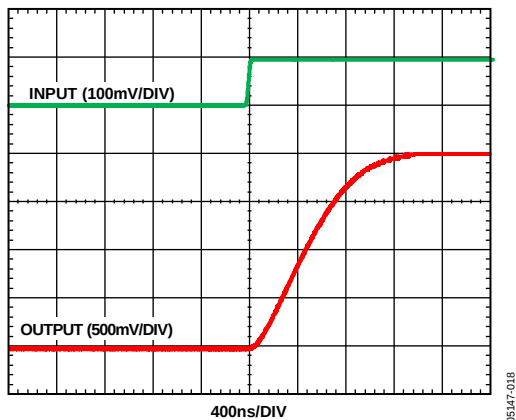
Figure 9. Rise Time
