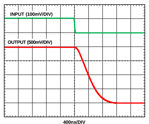
Figure 8. Fall Time
