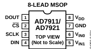
Figure 9. 8-Lead MSOP Pin Configuration
