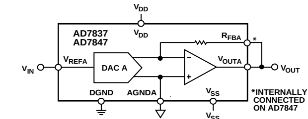
Figure 15. Unipolar Binary Operation
