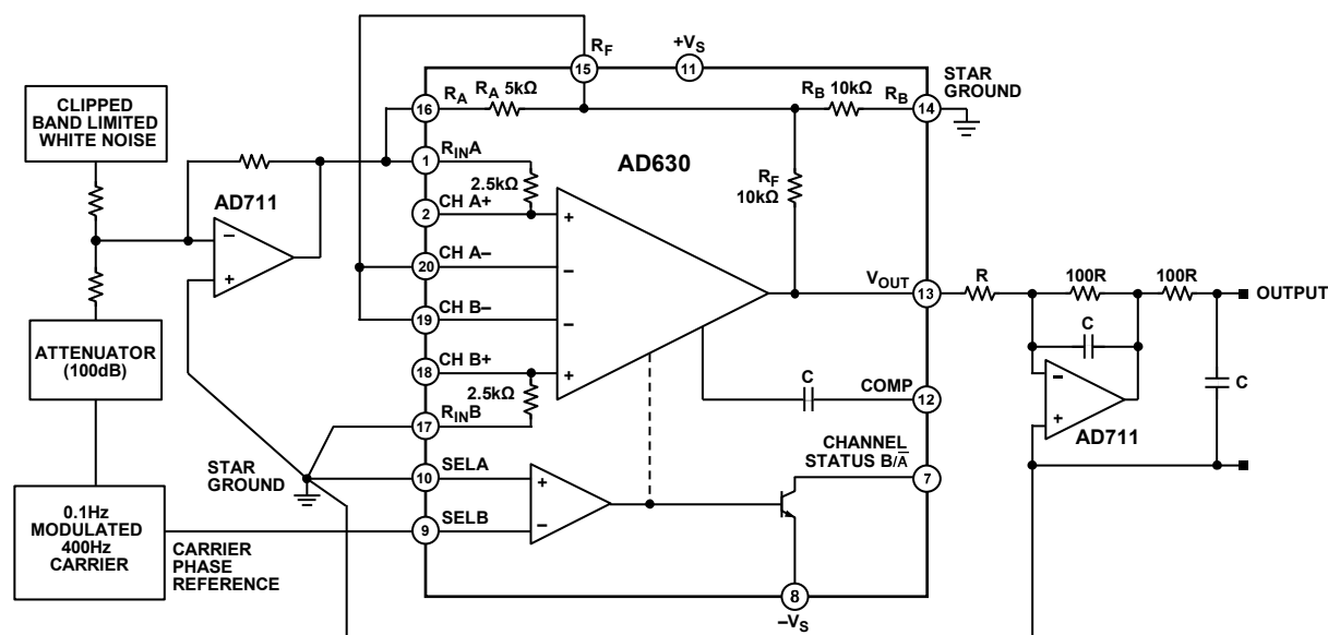
Figure 35. Lock-In Amplifier
