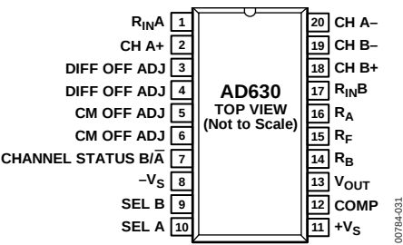
Figure 4. 20-Lead PDIP Pin Configuration
