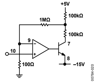
Figure 26. Comparator Hysteresis
