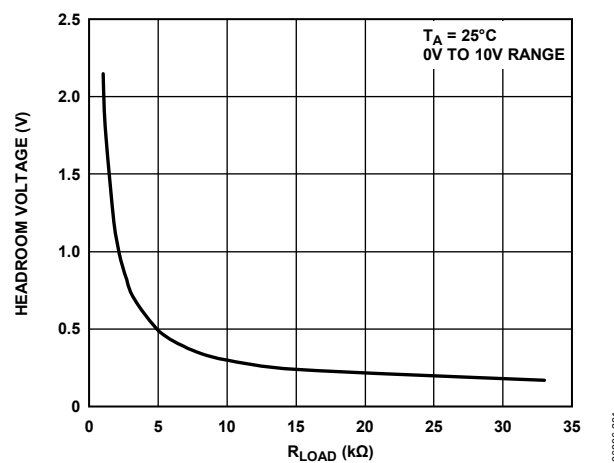
Figure 34. V_{OUT} Headroom
