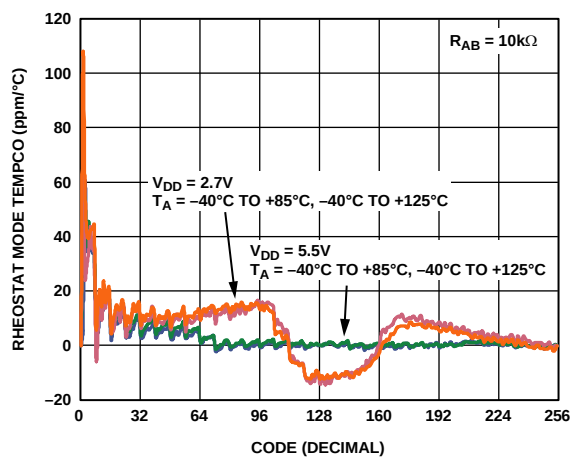
Figure 17. Rheostat Mode Tempco \Delta R_{WB}/\Delta T vs. Code
