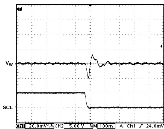
Figure 25. Digital Feedthrough
