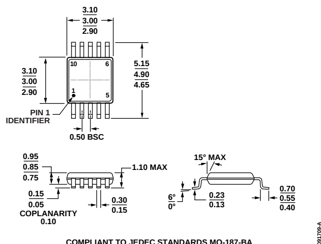
Figure 69. 10-Lead Mini Small Outline Package [MSOP] (RM-10)
