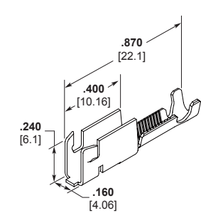
D AMPLIVAR Direct Connect Contact
