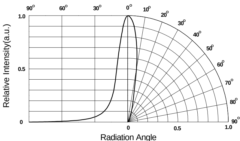
Radiation Characteristics
