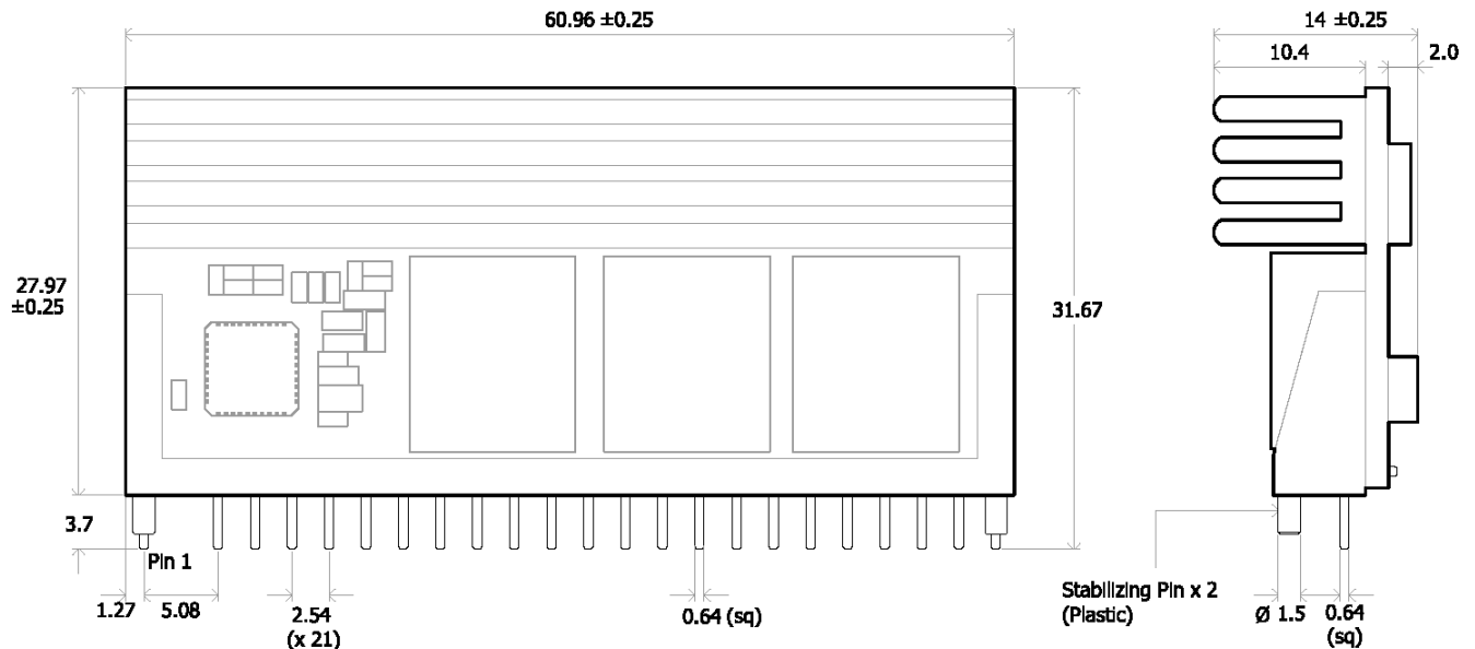
Figure 48. Mechanical Drawing
