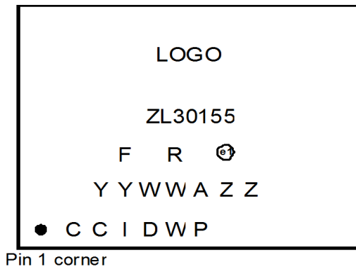
Figure 35 - Custom Factory Programmed Device Top Mark
