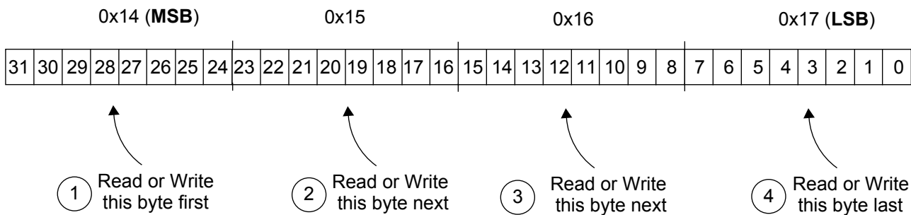
Figure 26 - Accessing Multi-byte Register Values
