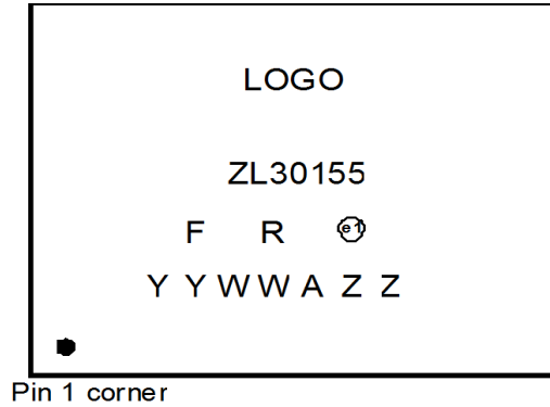
Figure 34 - Non-customized Device Top Mark
