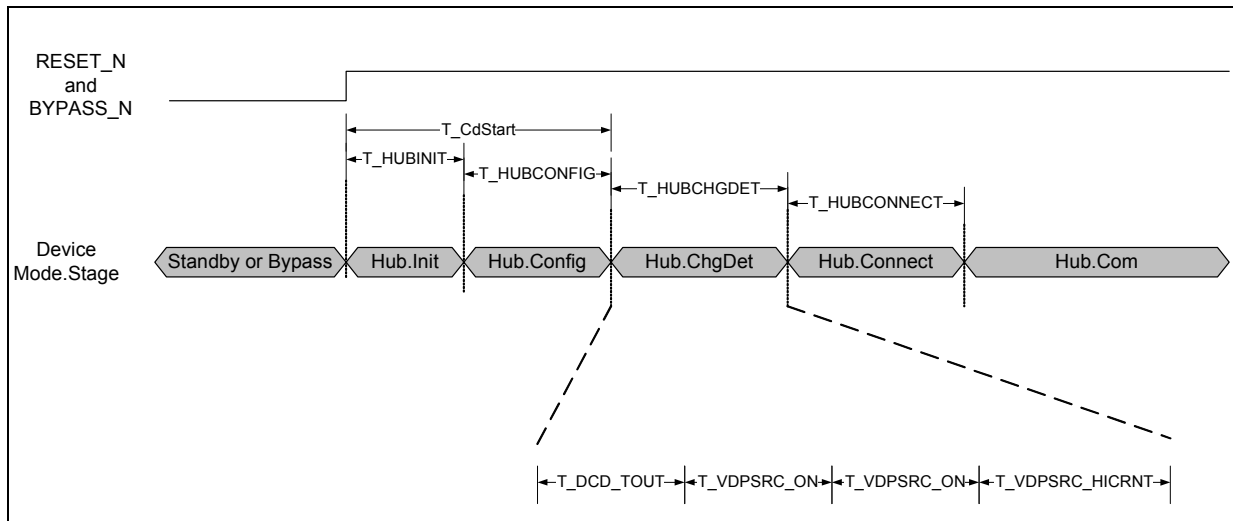
FIGURE 4-2: TIMING DIAGRAM FOR HUB STAGES
