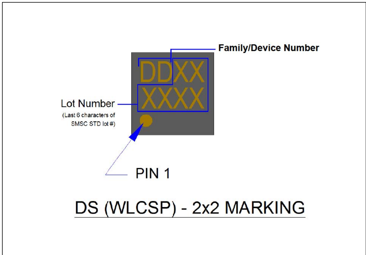
FIGURE 12-6: PACKAGE MARKING
