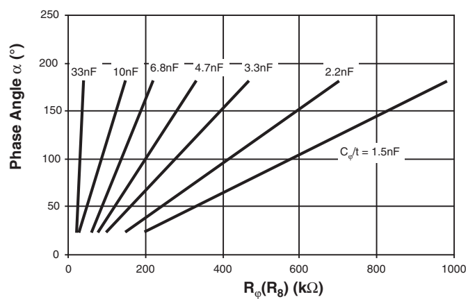
Figure 5-1. Ramp Control
