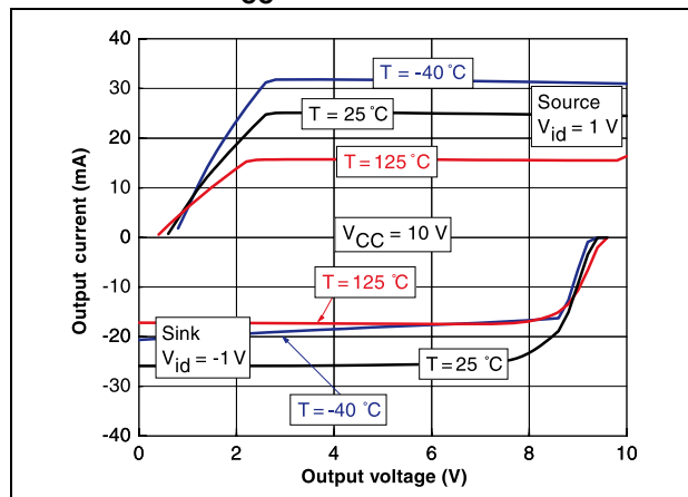
Figure 14. Output current vs. output voltage at V_{CC} = 10\text{ V}
