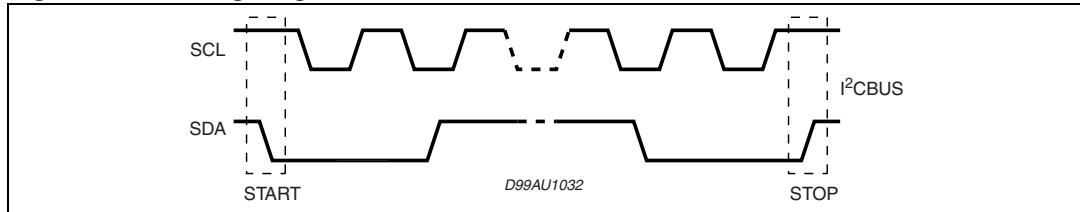
Figure 21. Timing diagram of S-bus and I 2 C bus
