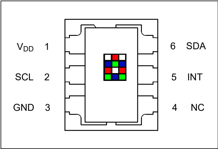
Figure 3: Pin Diagram
