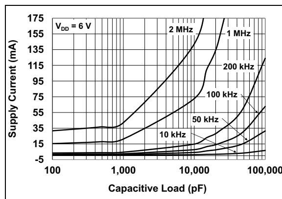
FIGURE 2-18: Supply Current vs. Capacitive Load ( V_{DD} = 6\text{V} ).
