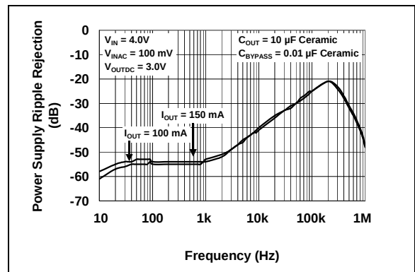
FIGURE 2-24: PSRR vs. Frequency ( C_{OUT} = 10 \mu F Ceramic).
