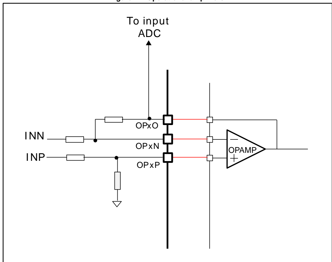
Figure 14: Operational amplifiers
