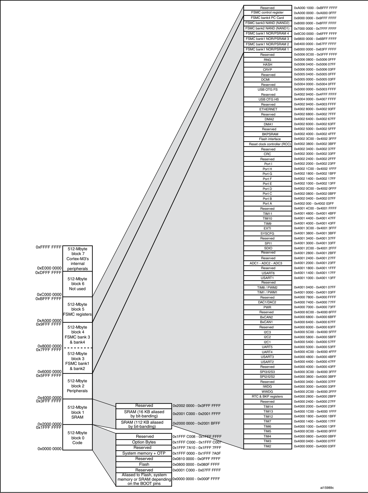
Figure 14. Memory map
