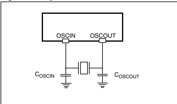
Figure 16. Crystal Resonator
