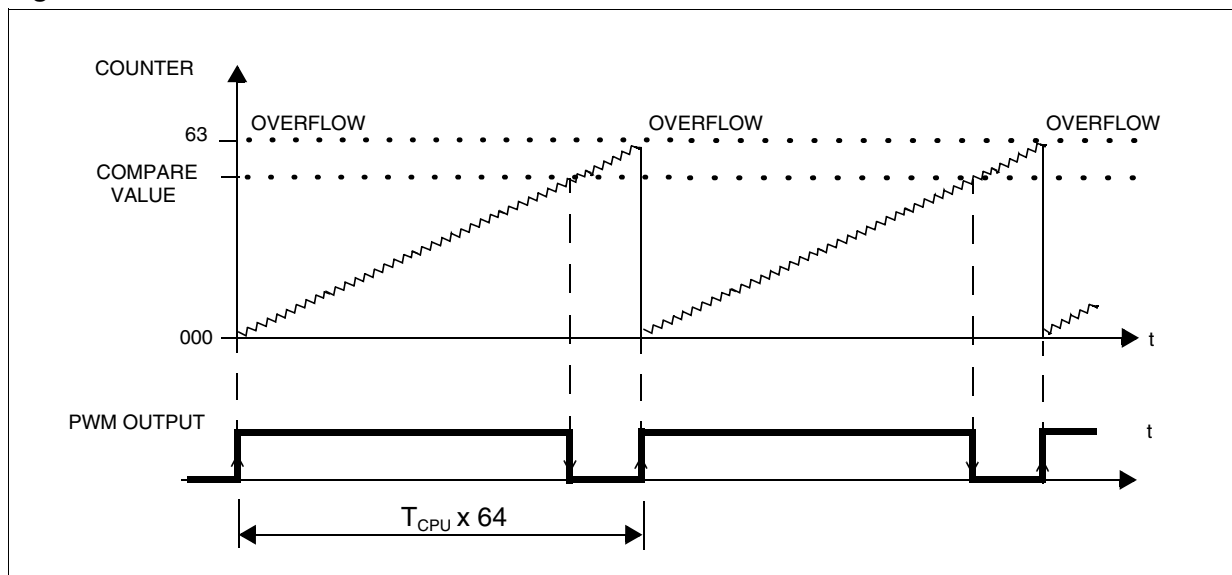
Figure 48. PWM Generation
