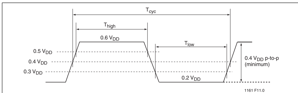
Figure 8: CLK Waveform
