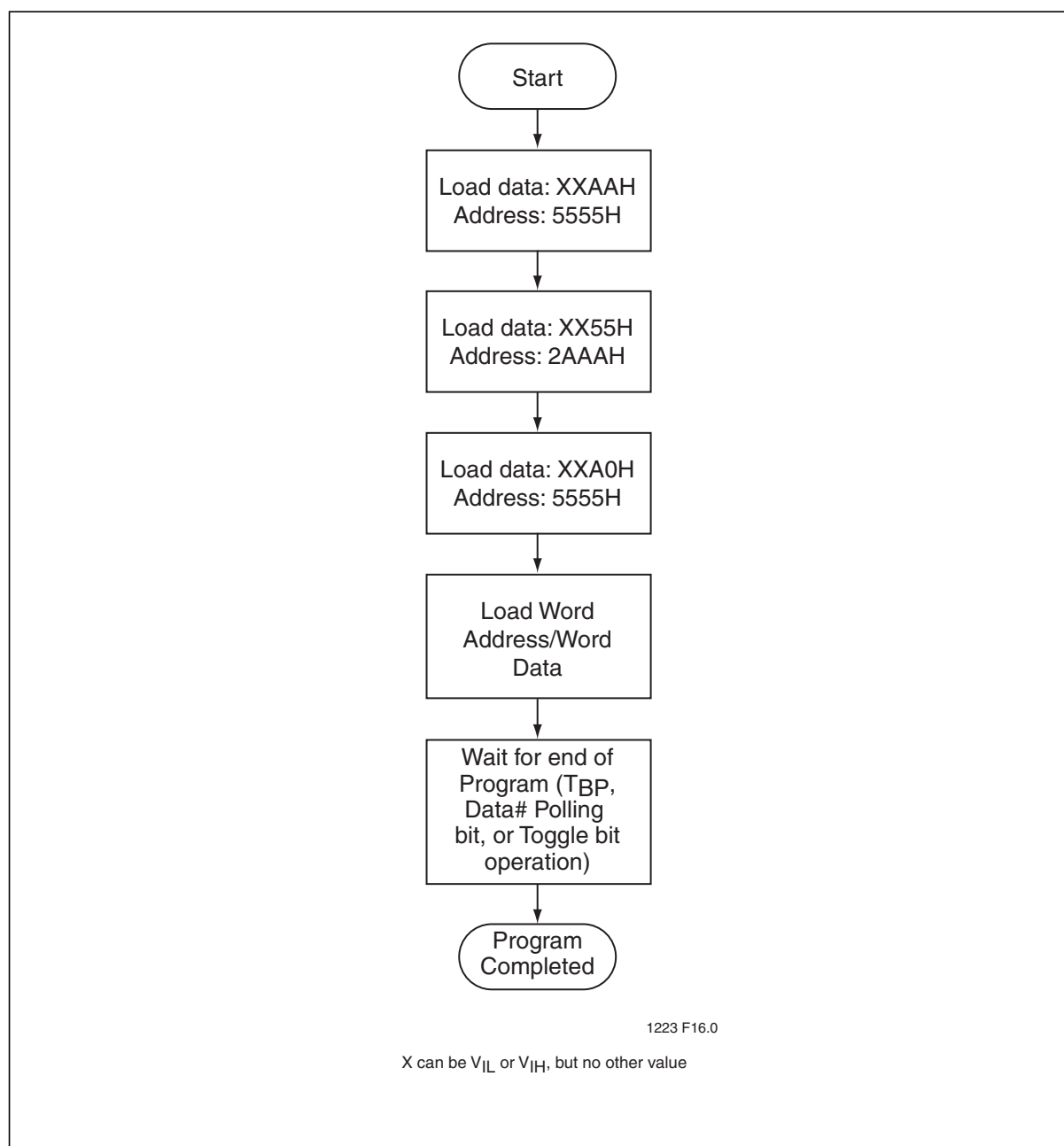
Figure 20: Word-Program Algorithm
