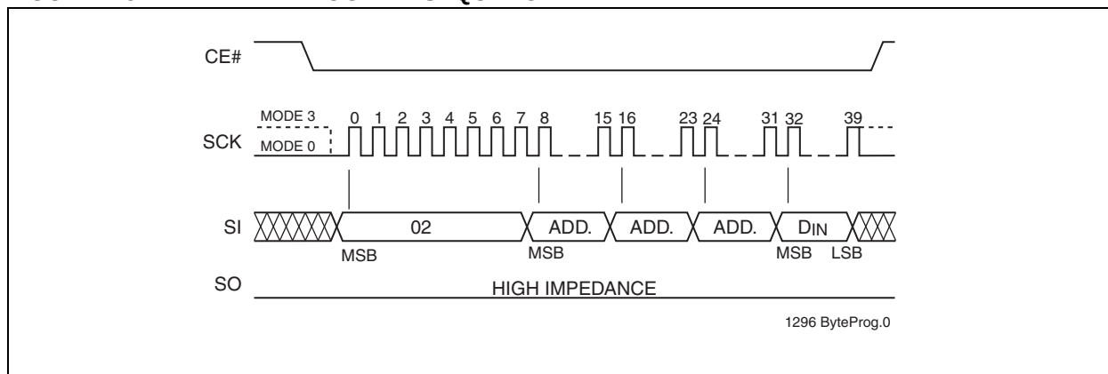
FIGURE 4-5: BYTE-PROGRAM SEQUENCE
