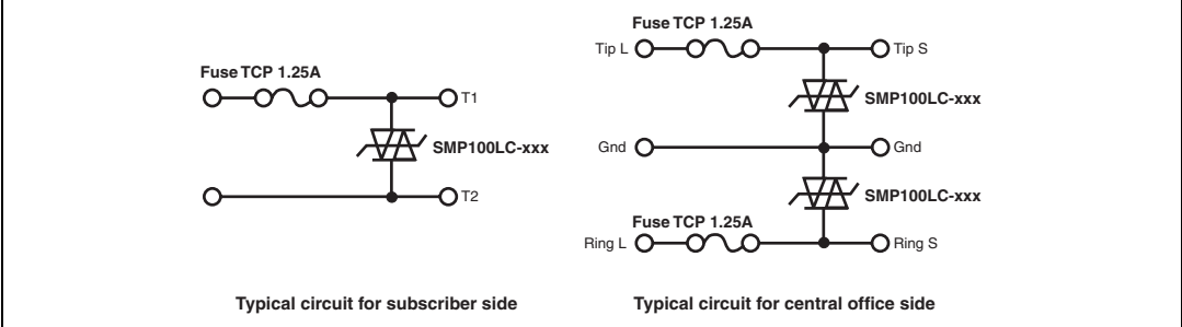
Figure 11. Typical circuits
