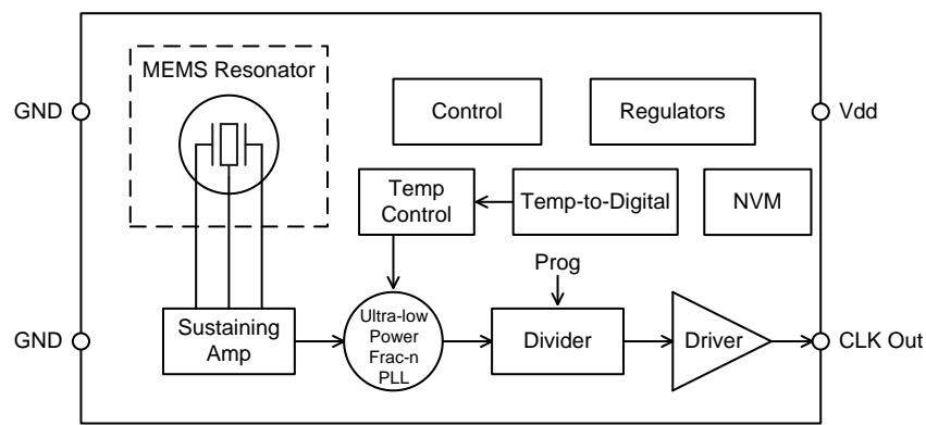
Figure 2. SiT1552 Block Diagram
