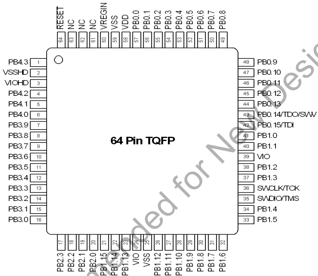
Figure 6.3. SiM3C1x6-GQ Pinout
