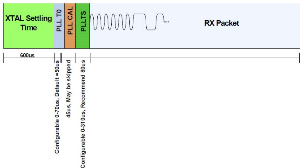
Figure 7. RX Timing
