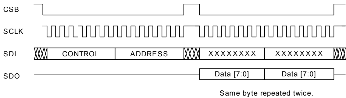
Figure 40. Read Operation via a 16-bit SPI Port
