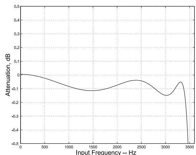
Figure 12. IIR Receive Filter Passband Ripple
