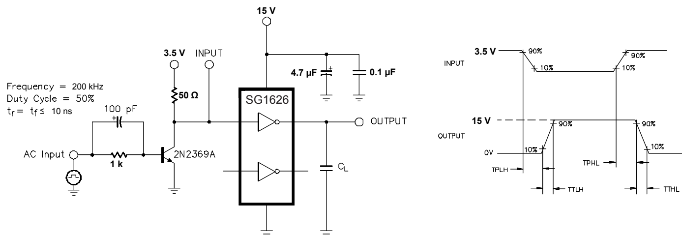
Figure 1 · AC Test Circuit and Switching Time Waveforms
