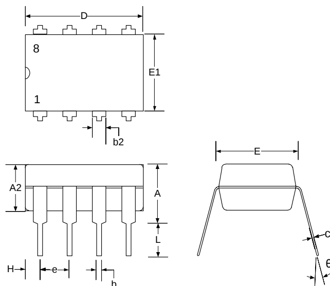
Figure 17 • M 8-Pin PDIP Package Dimensions
