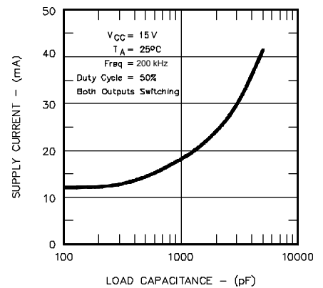
Figure 7 · Supply Current vs. Capacitive Load
