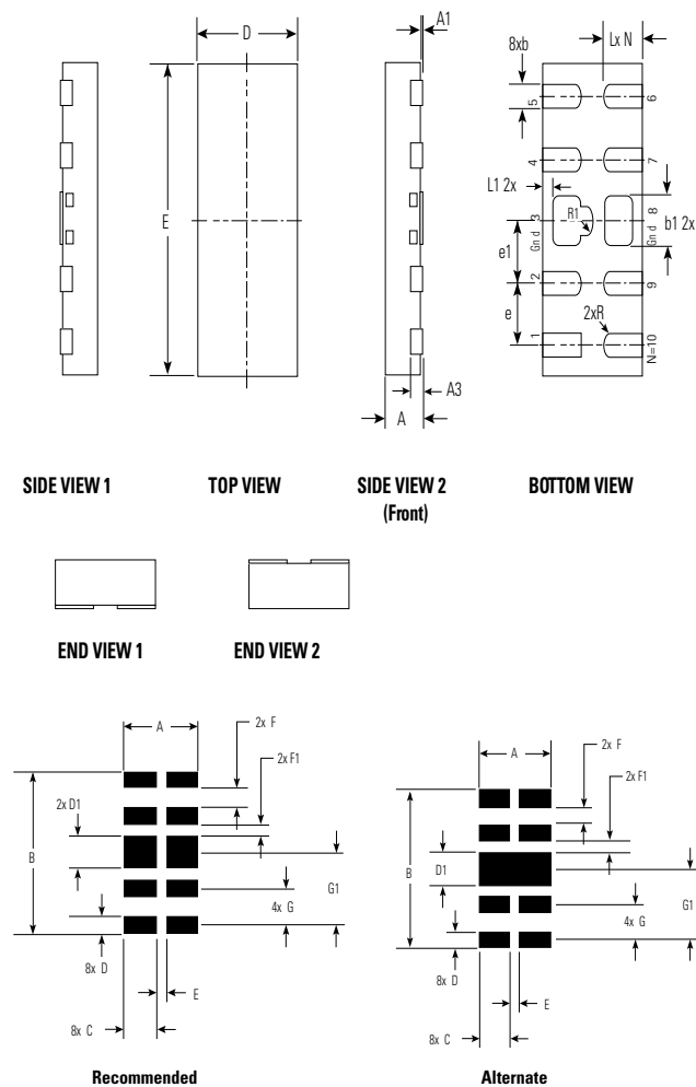
Pad Layout
