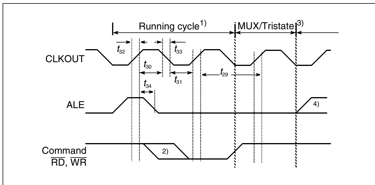
Figure 24 CLKOUT Timing
