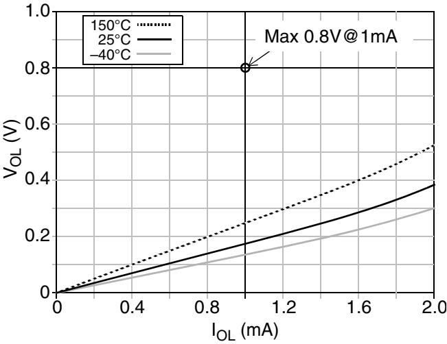
b) V_{DD} = 3V , Low Drive
