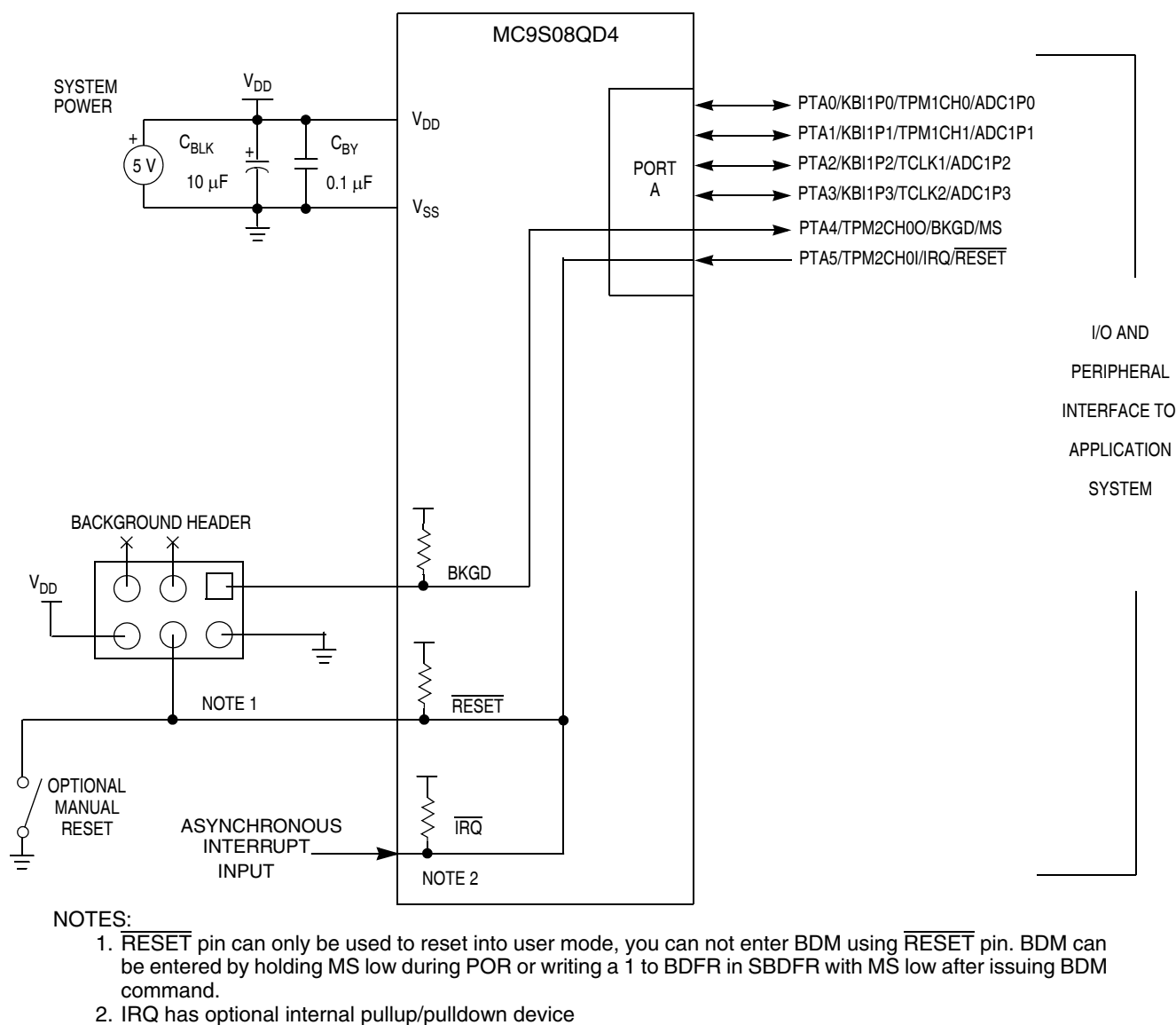
Figure 2-2. Basic System Connections
