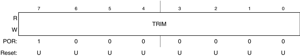
Figure 9-5. ICS Trim Register (ICSTRM)
