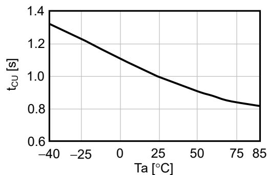
2. 12 t_{CU} vs. T_a
