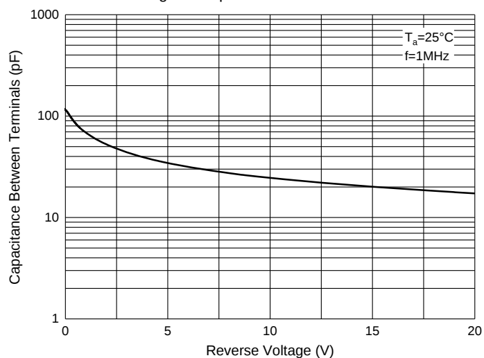
Fig. 3 - Capacitance Characteristics
