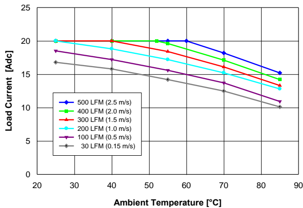
Fig. 1: Available load current vs. ambient air temperature and airflow rates for converter with G height pins mounted vertically with air flowing from pin 1 to pin 3, MOSFET temperature \leq 125 °C, V_{in} = 48 V.
