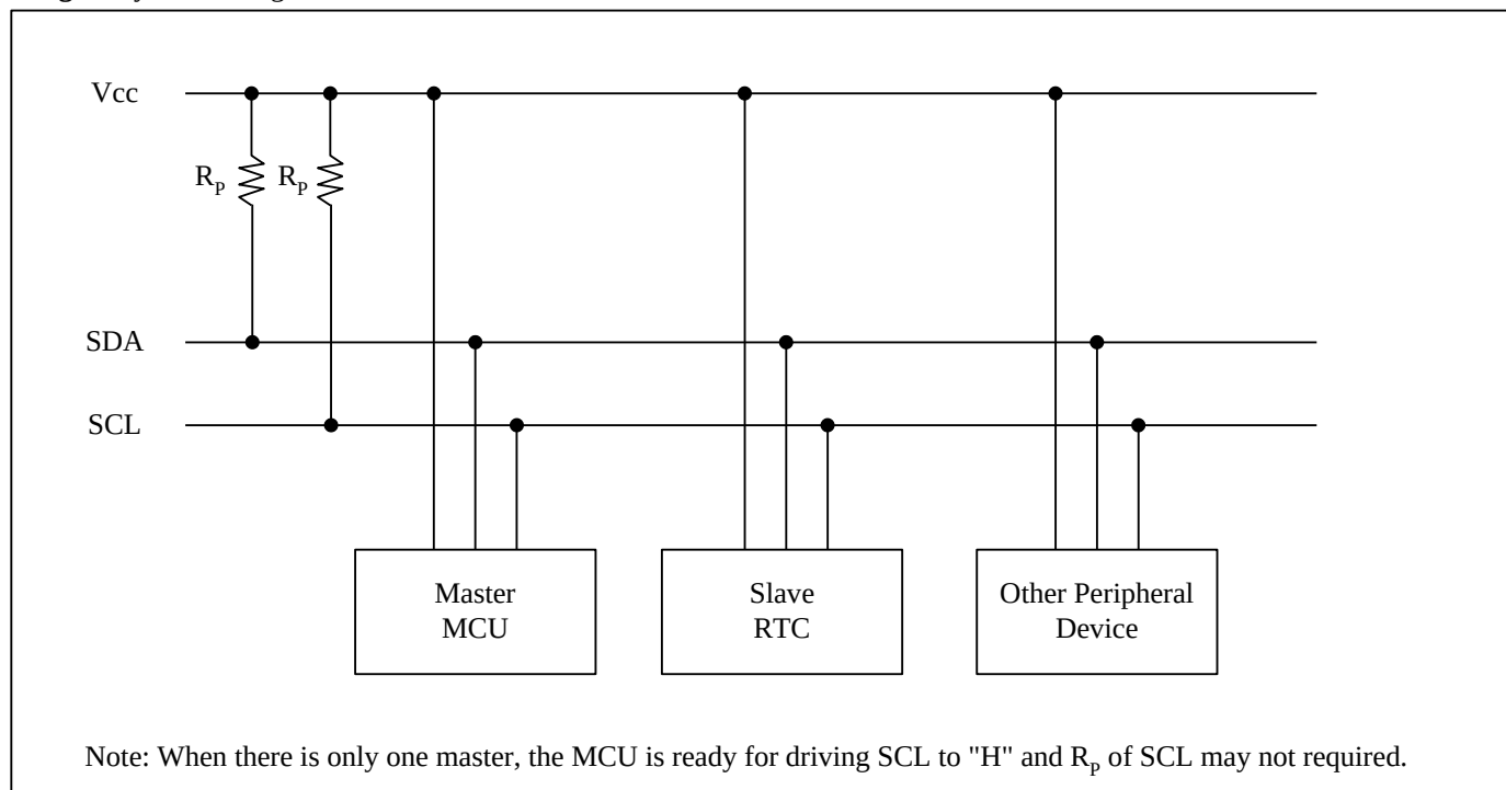
Fig 1. System configuration
