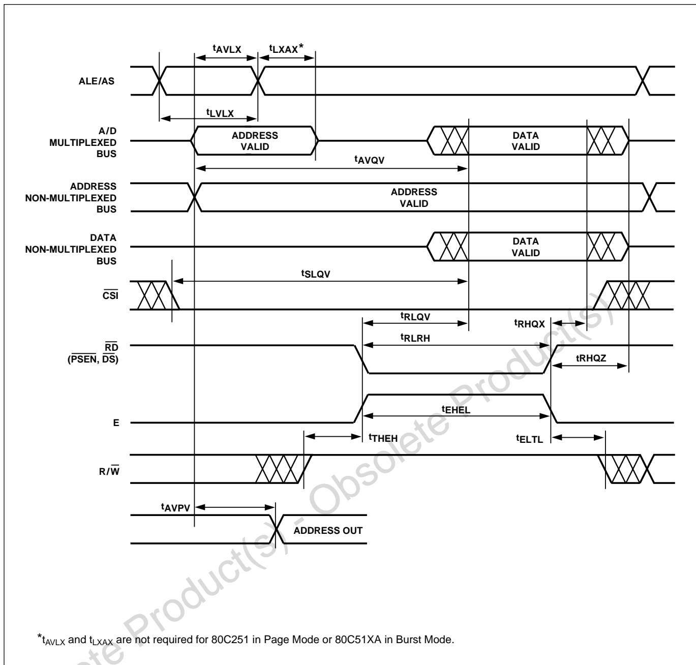
Figure 27. Read Timing
