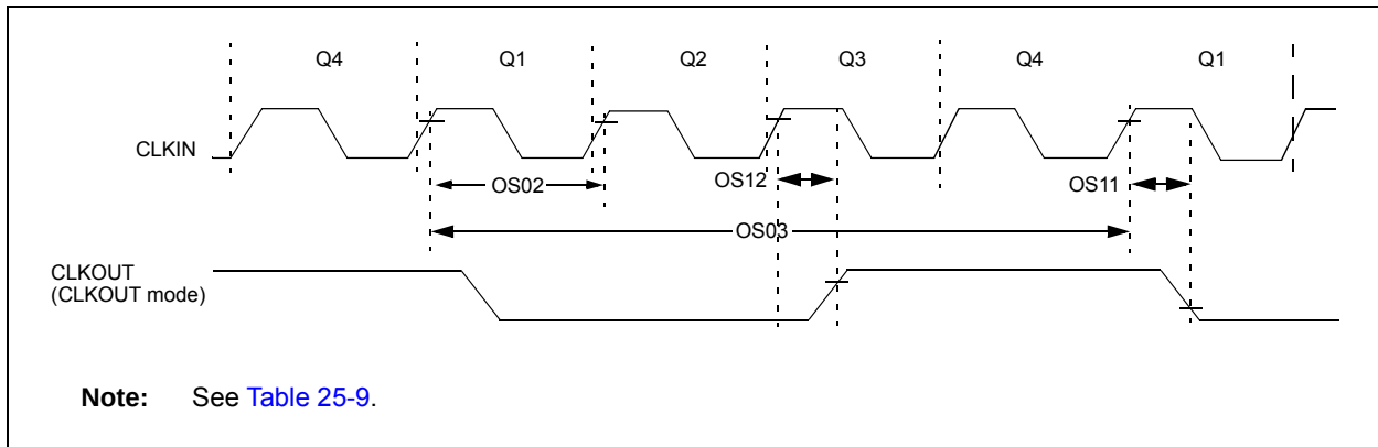
FIGURE 25-5: CLOCK TIMING
