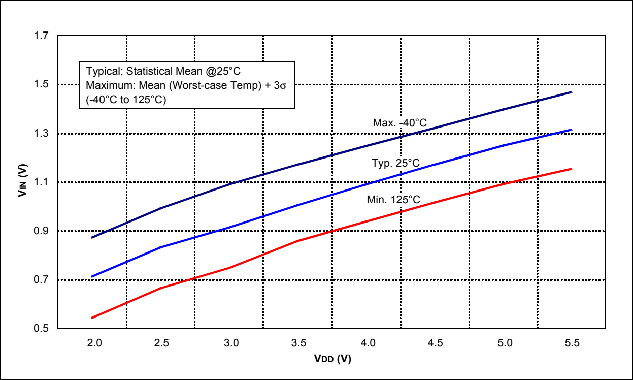
FIGURE 13-22: SCHMITT TRIGGER INPUT THRESHOLD VIN vs. VDD OVER TEMPERATURE
