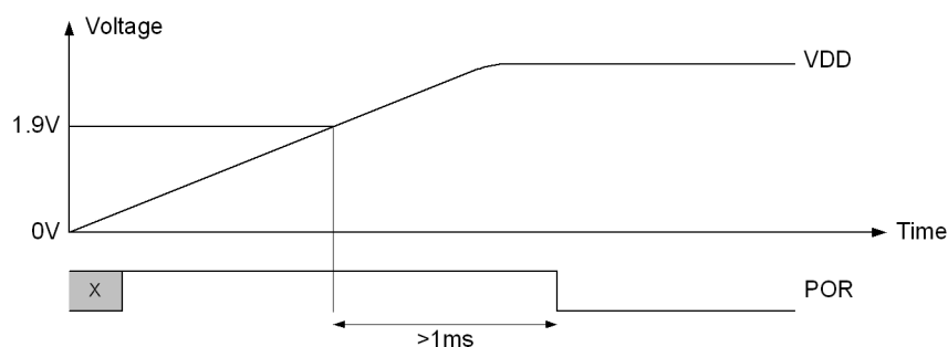
Figure 49. Power-on reset
