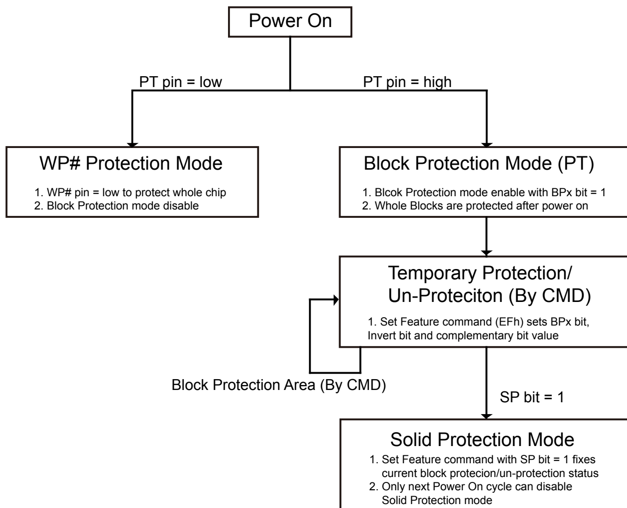
Figure 33. PT Pin and Block Protection Mode Operation
