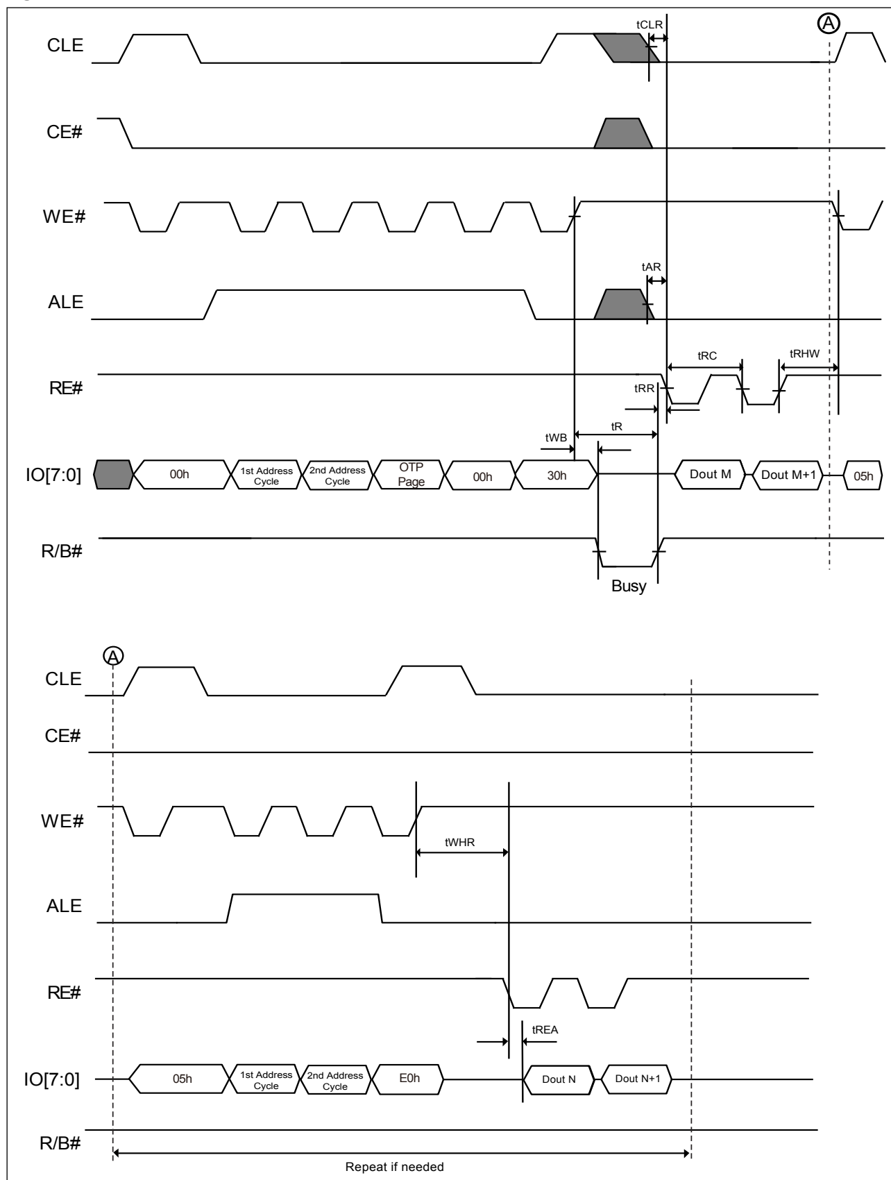
Figure 29. AC Waveforms for OTP Data Read with Random Data Output
