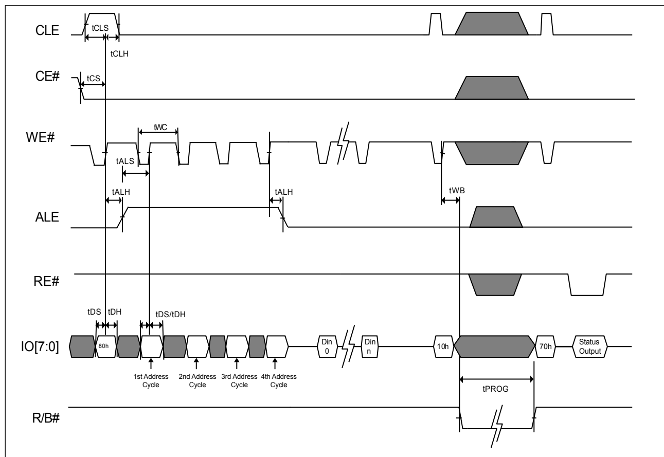
Figure 12. AC Waveforms for Program Operation after Command 80H
