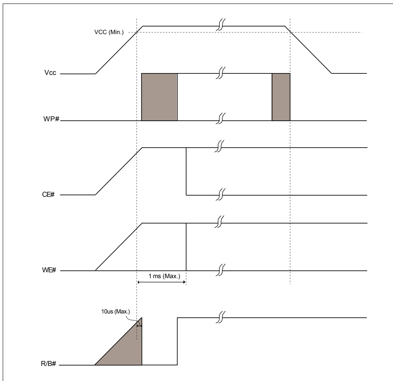
Figure 37. Power On/Off Sequence
