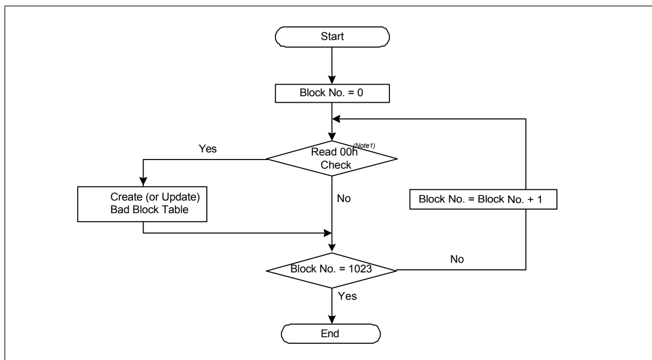
Figure 40. Bad Block Test Flow
