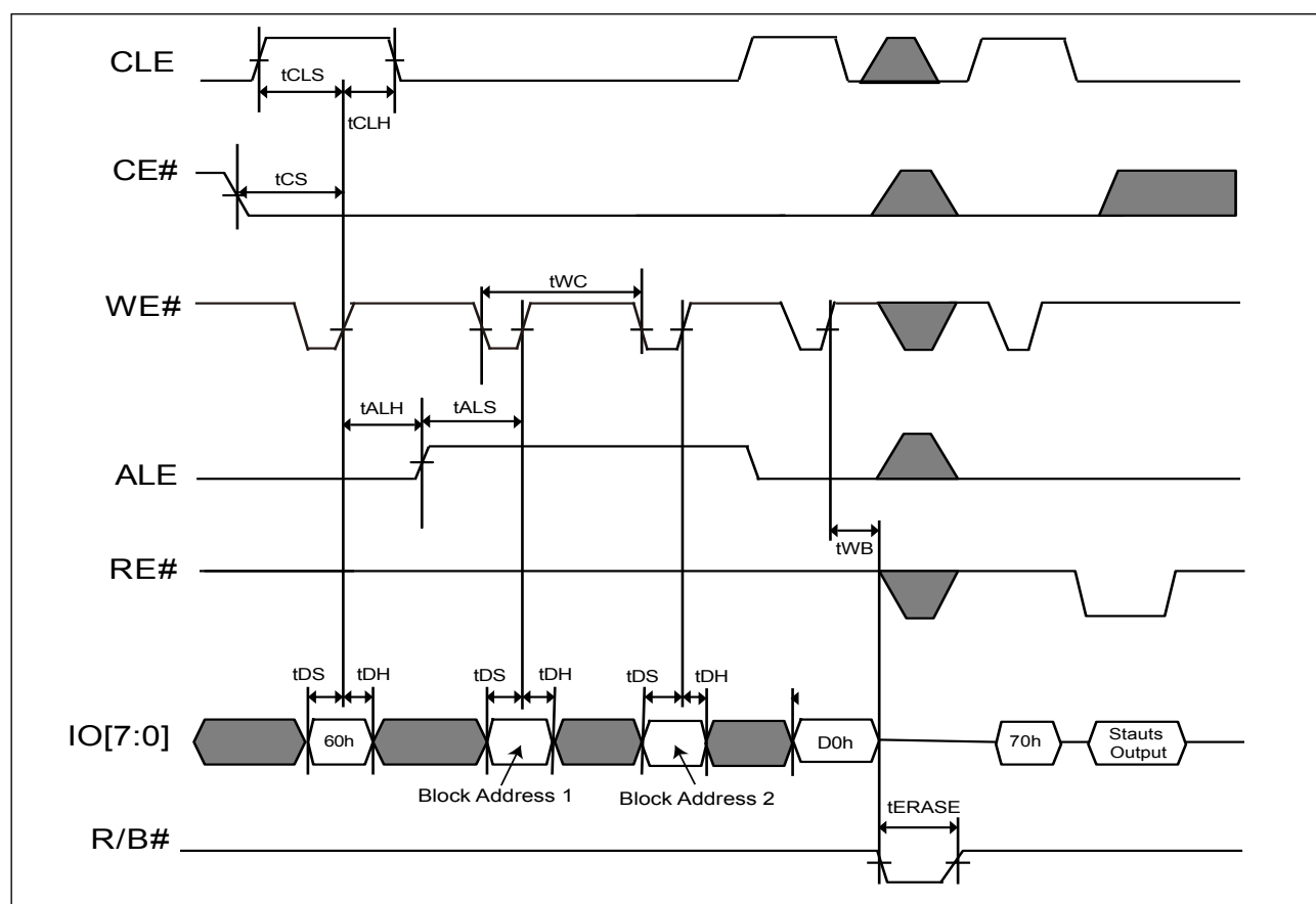
Figure 16. AC Waveforms for Erase Operation
