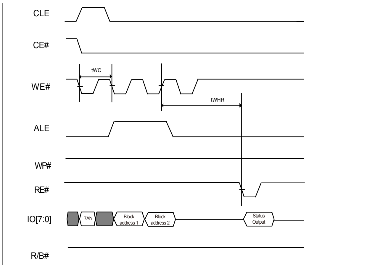
Figure 20. AC Waveforms for Block Protection Status Read
