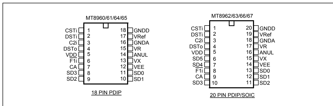
Figure 2 - Pin Connections
