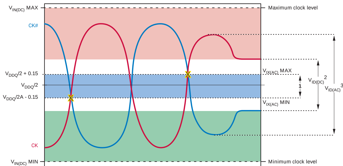
Figure 7: Clock Input
