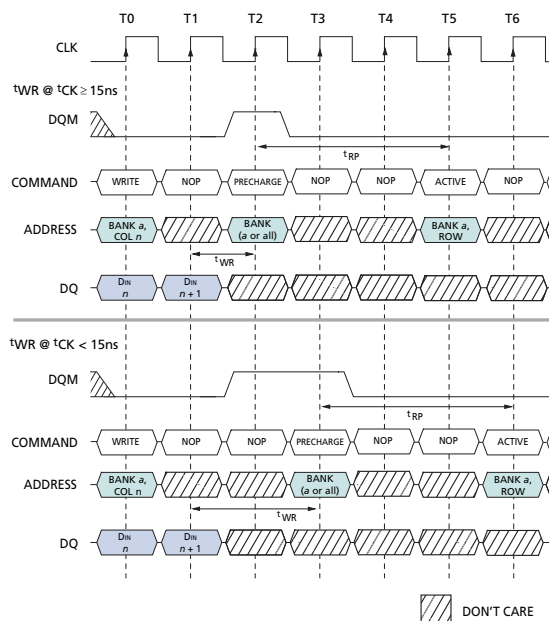
Figure 21: WRITE-To-PRECHARGE
