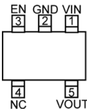
5-Pin SC-70 (C5) Fixed Version
